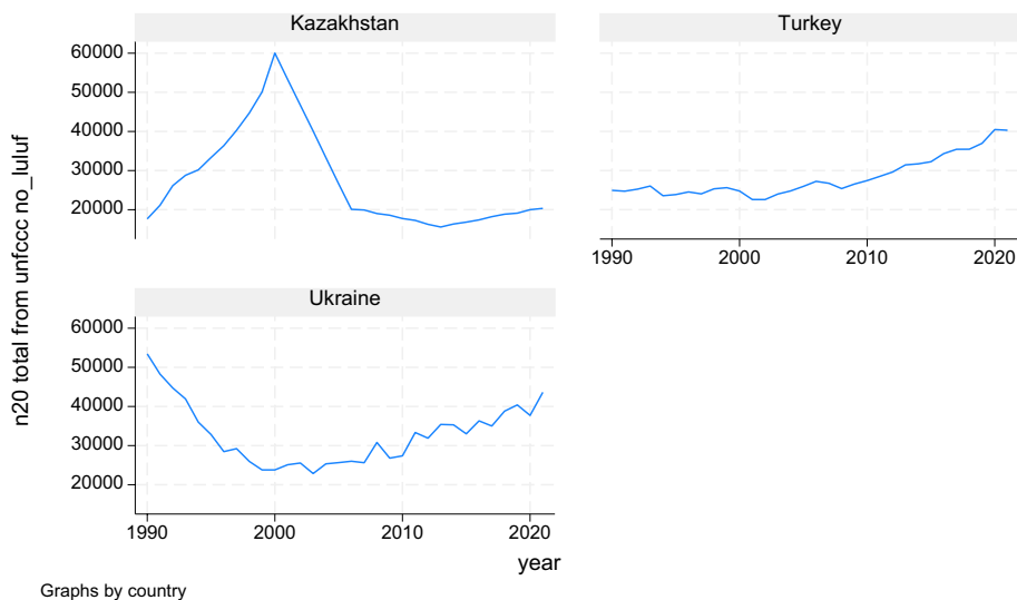
Fig. 11 Accelerating N 2 O emissions in several Annex I countries. Source Author's calculation of UNFCCC data
