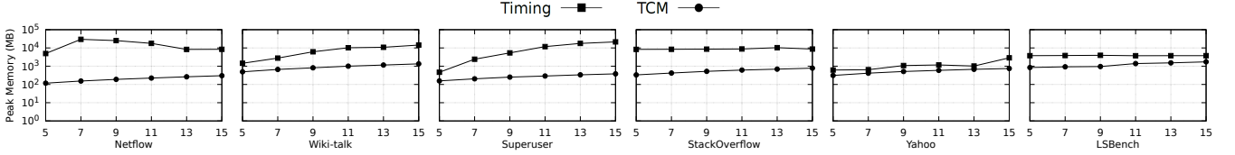
Fig. 10: Average peak memory for varying query size
