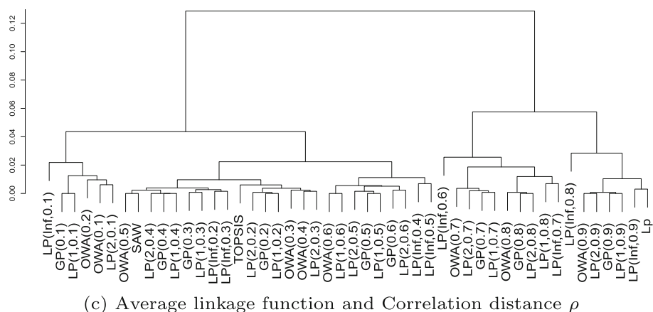
Fig. 15 Dendrogram results for Average linkage function and Manhattan distance, Maximum distance, Correlation distance \rho , which involves creating clusters that have a predetermined ordering from top to bottom
