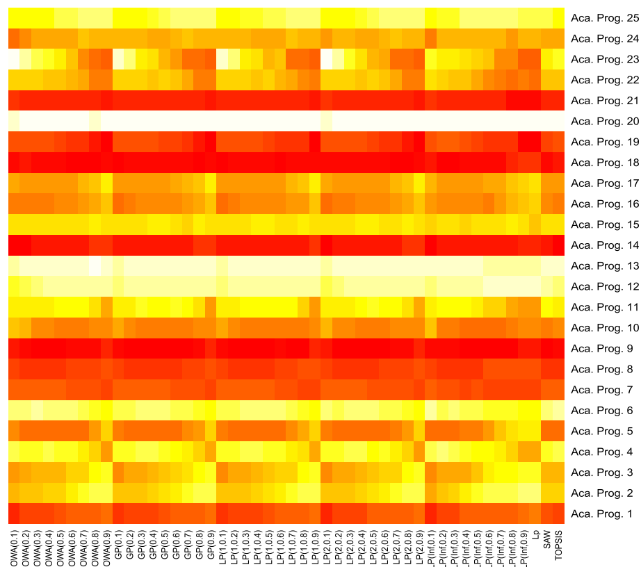
Fig. 3 The diagram of the values of the ranks obtained by different methods. The shading in the main panel goes from dark red (higher values) to very light yellow (lower values). (Color figure online)
