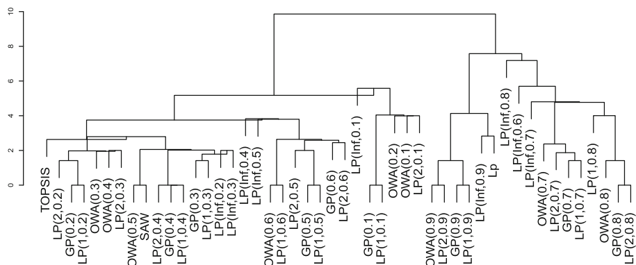
Fig. 12 Dendrogram for Centroid linkage function and Euclidian distance, which involves creating clusters that have a predetermined ordering from top to bottom
