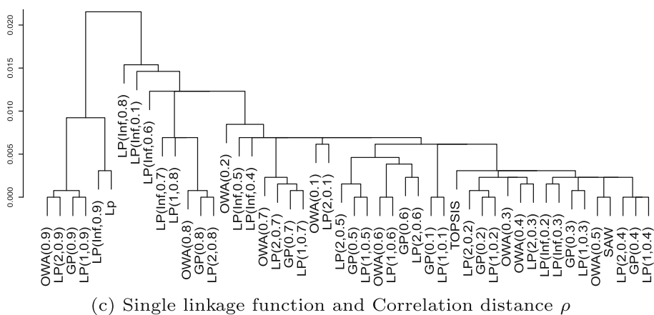
Fig. 13 Dendrogram results for Single linkage function and Manhattan distance, Maximum distance, Correlation distance \rho , which involves creating clusters that have a predetermined ordering from top to bottom
