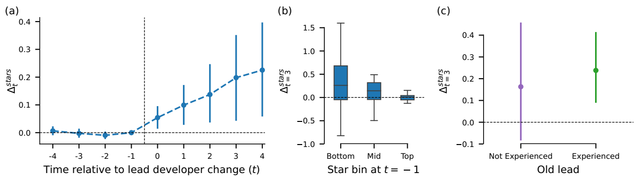
Fig. 4 | Lead developer changes are associated with faster success growth.
