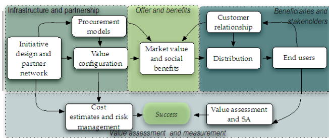
Fig. 1 PPBM framework
