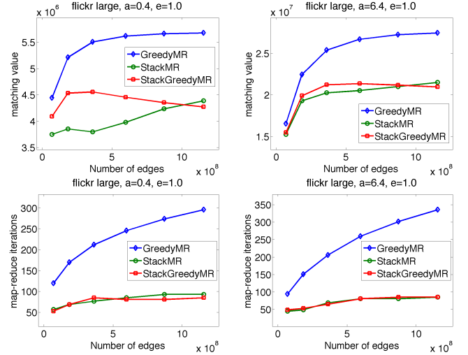
Figure 2: flickr-large dataset: matching value and number of iterations as a function of the number of edges.
