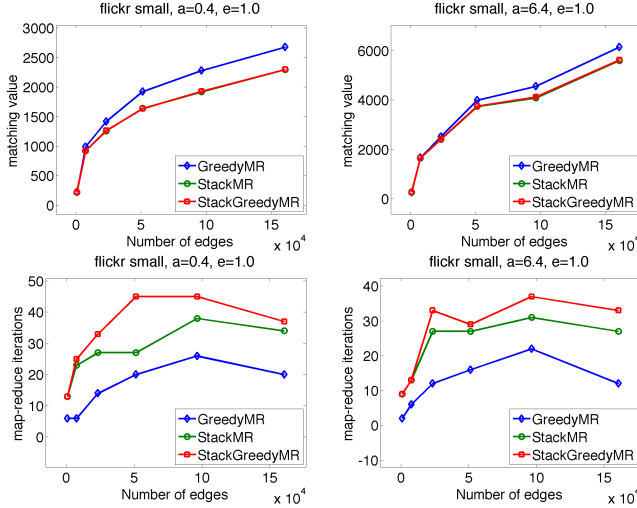
Figure 1: flickr-small dataset: matching value and number of iterations as a function of the number of edges.
