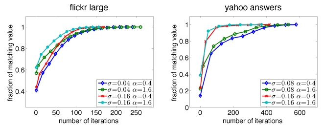
Figure 5: Value of the b -matching achieved by the GREEDYMR algorithm as a function of the number of MapReduce iterations. b -matching value is shown as a fraction of the final value achieved.
