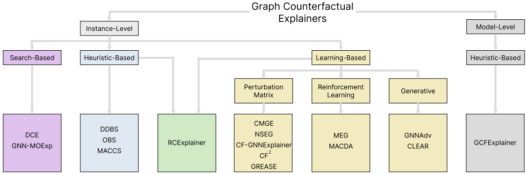
Fig. 2. Taxonomy of GCE methods.
