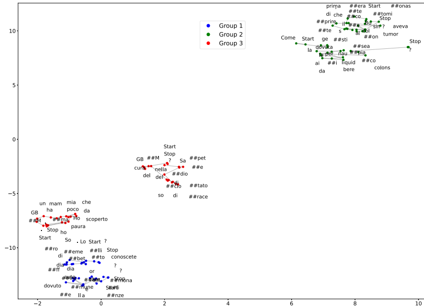
Fig. 5. t-SNE visualization of word contextual embeddings, obtained with BERT (Mdl21), of the tokens for 9 selected sentences – see Table IV.
